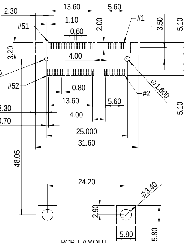
PCB LAYOUT
