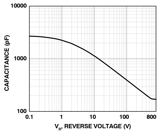
Figure 9. Capacitance vs. Reverse Voltage
