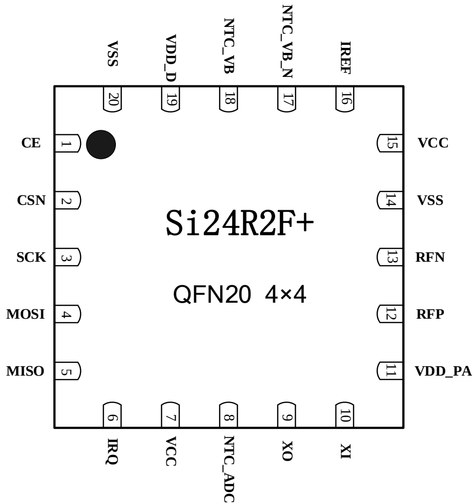
Figure 2-1 Si24R2F+ pin information (QFN20 4×4 package)
