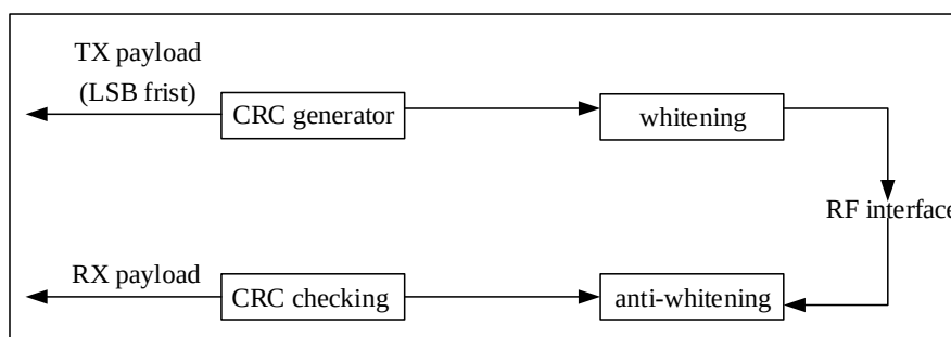
Figure 4-5 BLE packet data stream
