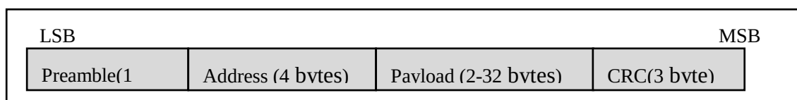
Figure 4-4 Bluetooth packet format
