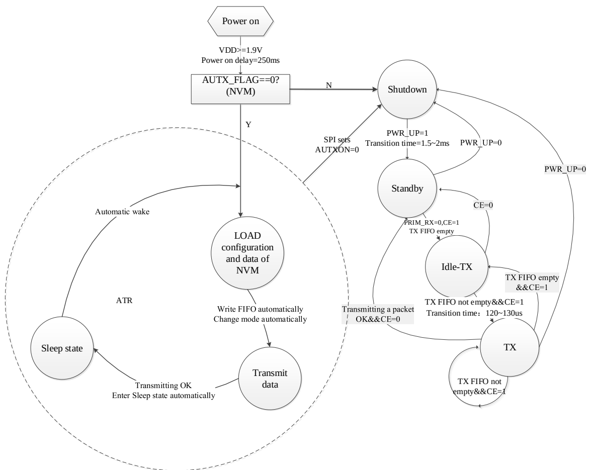
Figure 3-1 Si24R2F+ state control diagram
