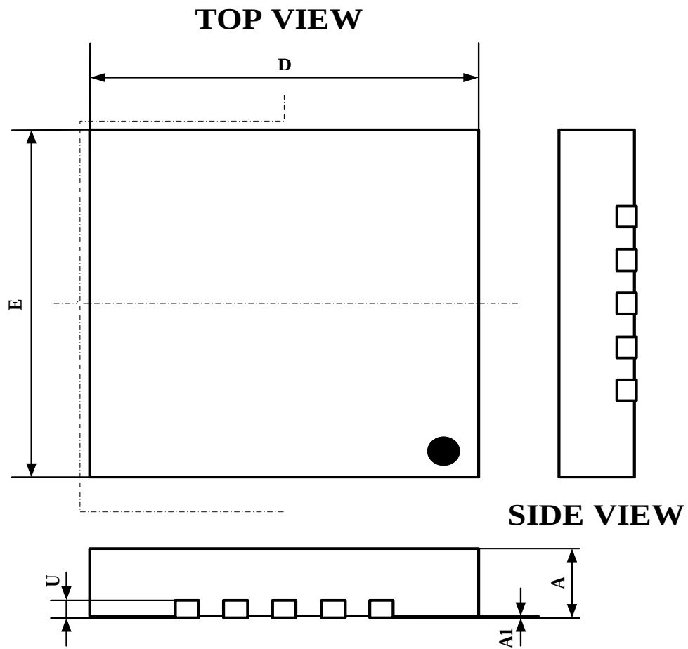
Figure 8-1 Top view
