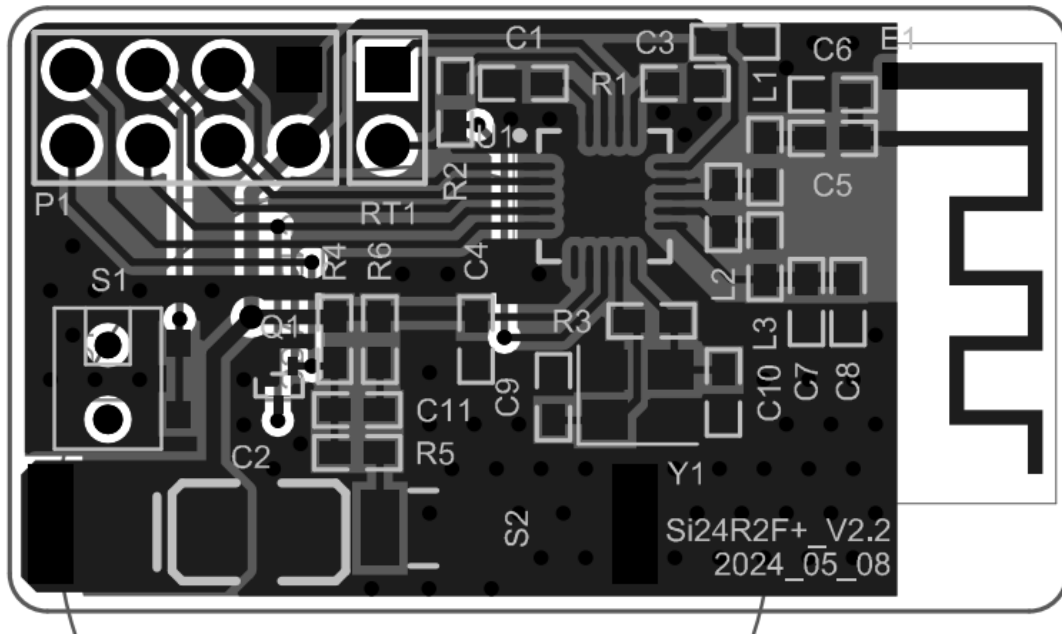
Figure 9-2 PCB layout
