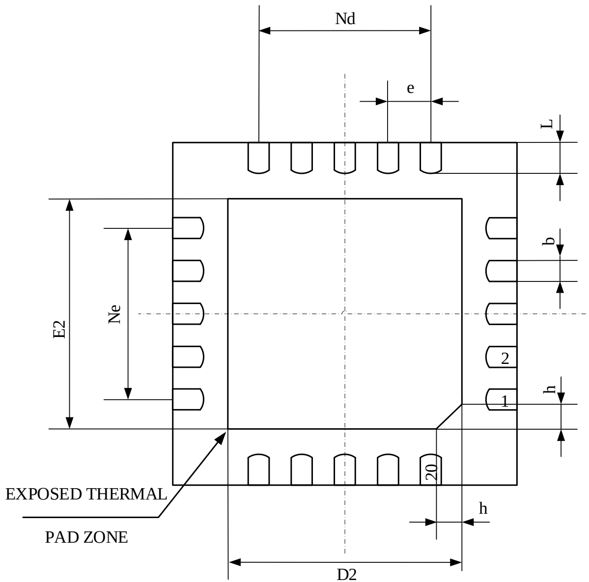
Figure 8-2 Package measurement (Top view)
