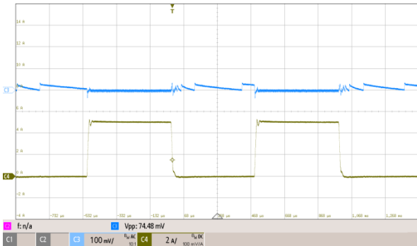
CH3: V_{OUT(AC)} CH4: I_{LOAD}
