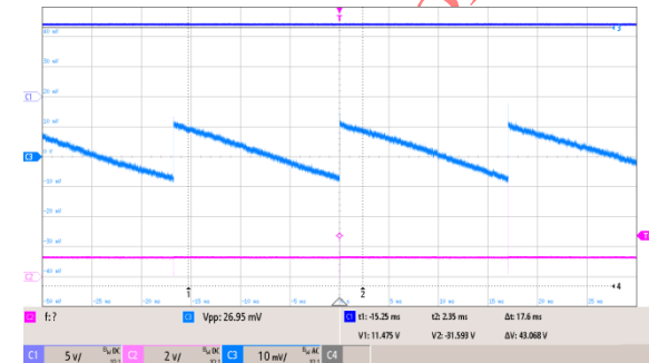
CH1: V_{PWR} CH2: V_{SW} CH3: V_{OUT(AC)}
