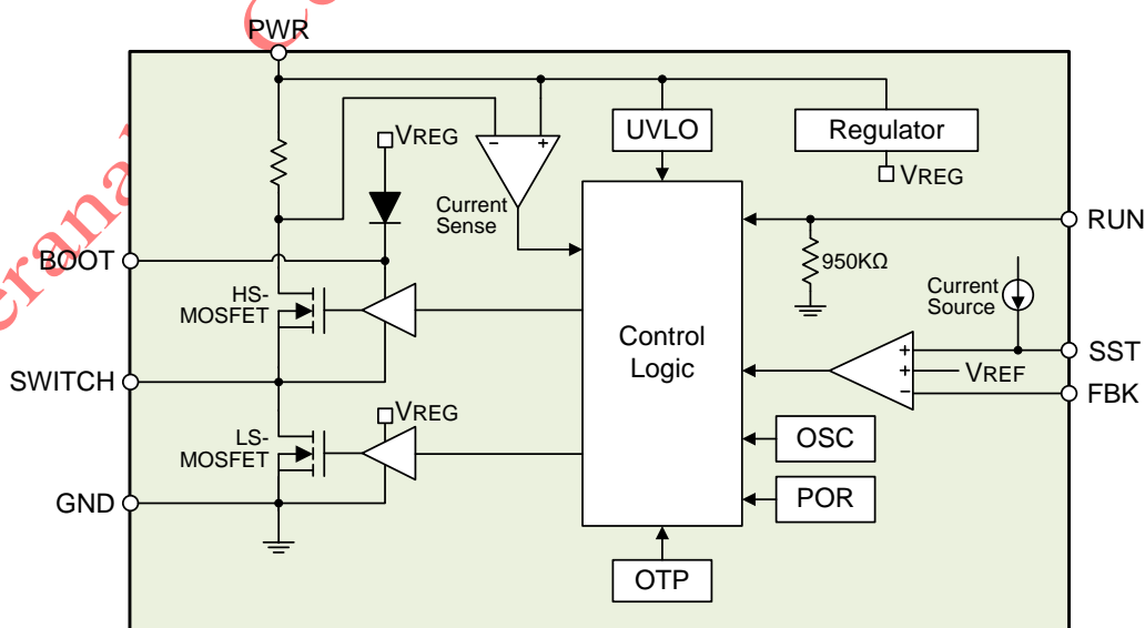
Figure 1. EA8276 internal function block diagram
